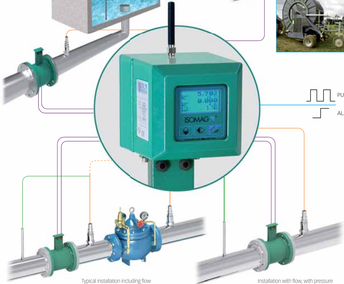
Typical installation including flow and pressure measurements to control PRV valve
